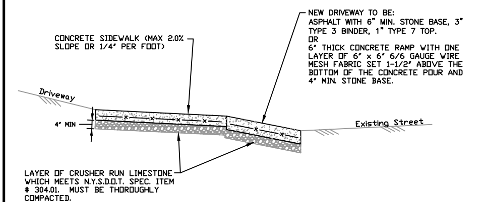
CROSS SECTION
