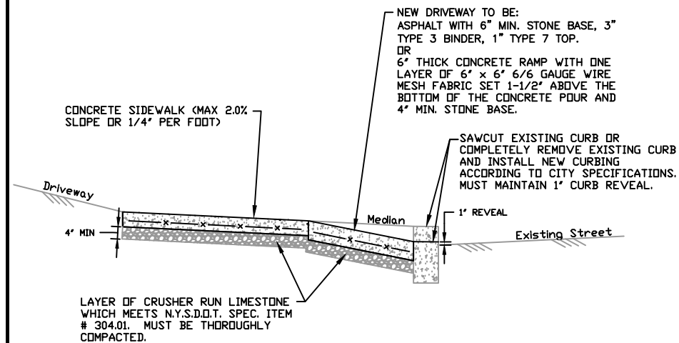
CROSS SECTION
